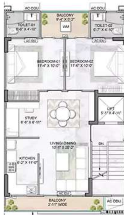
TYPICAL FLOOR
